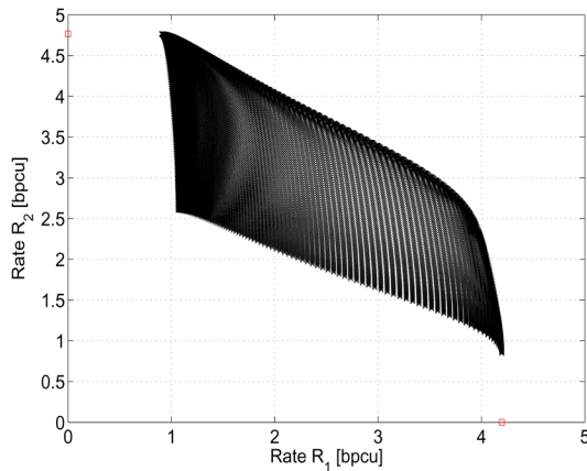
Fig. 2. Pareto boundary for a sample channel realization with N = 2 two transmit antennas at high SNR 30 dB.
